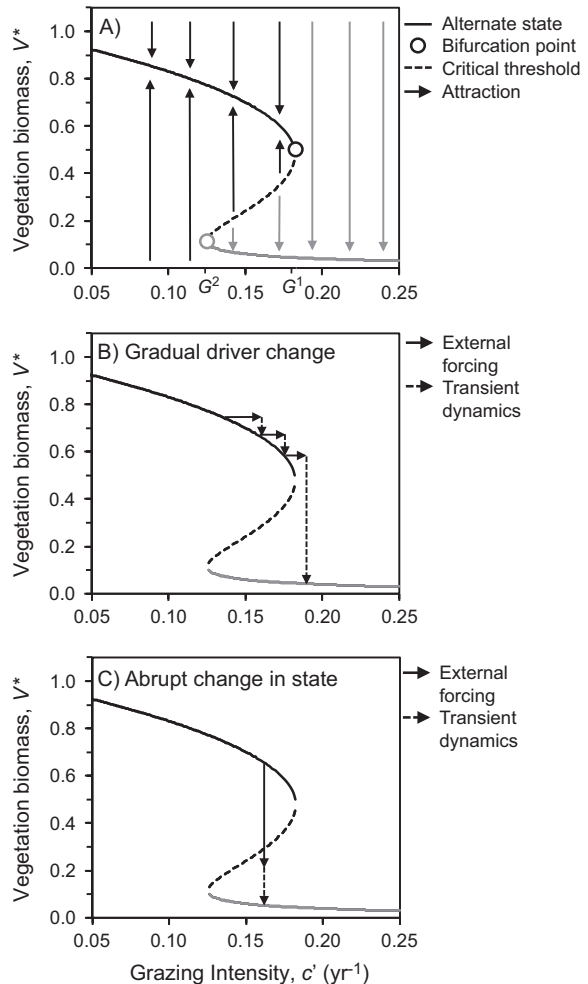
FIG. 2. (A) A fold bifurcation, with two alternative states: a high biomass state (the upper, solid black line) and the a low biomass state (lower, solid gray line). The two alternative states are attractors to which the system tends to converge. Arrows show the trajectory of the ecosystem for different initial conditions. The unstable equilibria (the dotted line), marks the boundaries of the two alternative states. At this boundary, small changes in state can force the system to the upper or lower state. The point G^1 is a bifurcation point, where the system goes from both the lower and upper state being stable, to only the lower state being stable. The system will start to transition to the upper state if the driver variable is reduced to the second bifurcation point, G^2 . (B and C) Different types of transitions from one alternative state to another. In both panels, the solid arrows represent changes in driver variables, and dashed arrows show transient dynamics. In panel B, the driver variable increases gradually until exceeding a bifurcation point. In panel C, an event alters the state variable, bringing it below a critical threshold. This specific fold bifurcation is generated using the default parameters of the model (Appendix S1).
